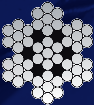
CONSTRUCTION 7X7 / TENSILE STRENGTH 1770N/MM2
