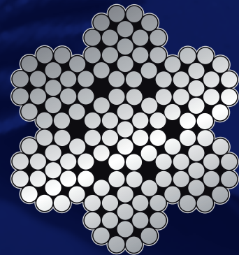
CONSTRUCTION 7X19 / TENSILE STRENGTH 1770N/MM2
